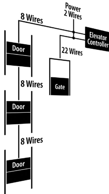
Figure 4: Connections of the wireless freight-elevator door system
