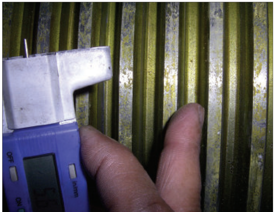
Annual check of groove profile
