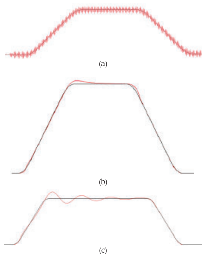
Figure 5: Speed control responses: (a) Proportional gain too high, inducing vibration; (b) proportional gain too low, causing overshoot; (c) proportional gain too low and integral gain too high, resulting in ringing
